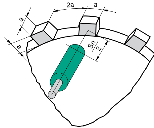
Actuator to determine the maximum switching frequency.
