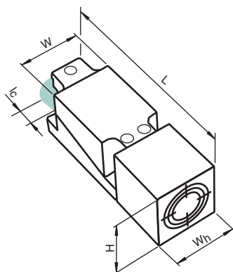
NJ20+U1+W-T
