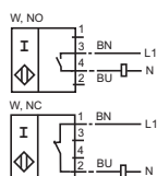
NJ20+U1+W-T
